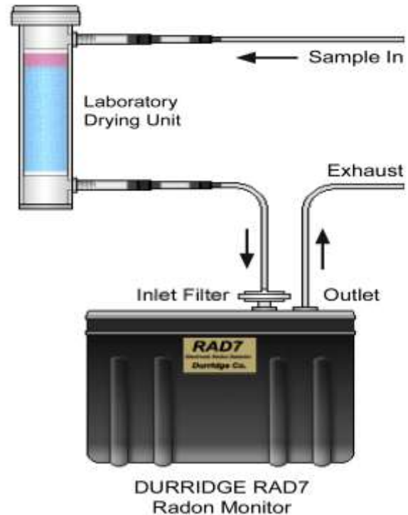
Figure 2: RAD7 Professional Electronic Radon Detector
