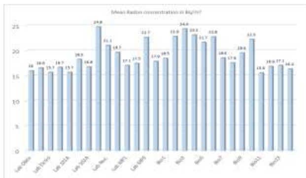
Fig 3: Mean Radon concentration in Bq/m 3
