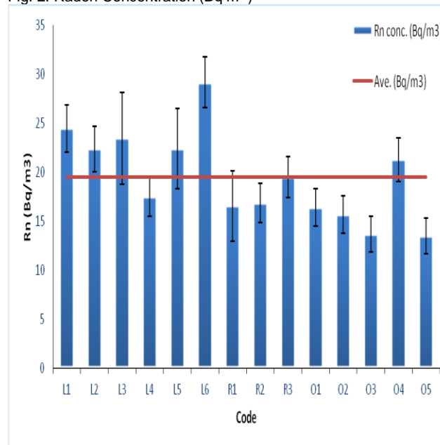
Fig. 2: Radon Concentration (Bq m -3 )
