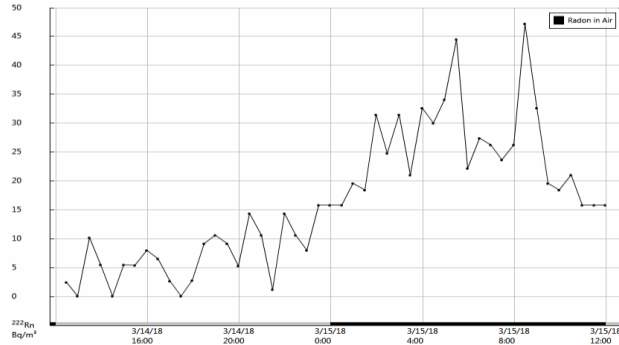
Fig. 3: Diurnal variation of radon in room (R2)
